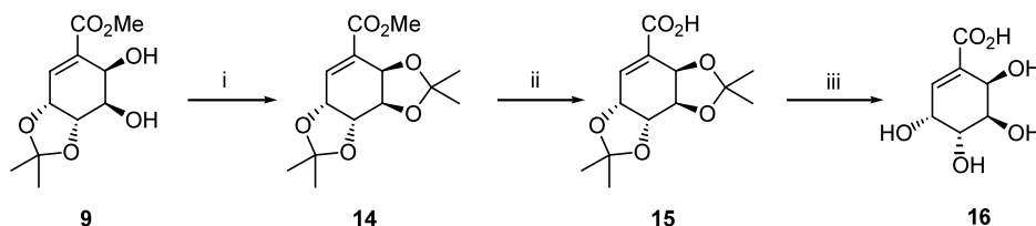
Scheme 3. Reagents and conditions: i, \text{CMe}_2(\text{OMe})_2 , CSA, rt, 3 h, 98%; ii, LiOH, THF– \text{H}_2\text{O} (1:4), rt, 1 h, 99%; iii, aq. HCl, MeOH, 30 h, 91%.
