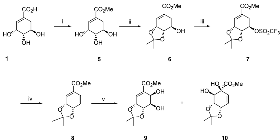
Scheme 1. Reagents and conditions: i, CSA, MeOH, reflux, 10 h, 96%; ii, CMe 2 (OMe) 2 , CSA, rt, 2 h, 95%; iii, Tf 2 O, DMAP, pyridine, CH 2 Cl 2 , –40°C, 40 min, 98%; iv, CsOAc, DMF, rt, 2 h, 81%; v, OsO 4 , NMO, t -BuOH–H 2 O (10:1), 0°C to rt, 8 h, 38% for 9 , 35% for 10 .
