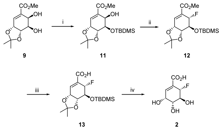
Scheme 2. Reagents and conditions: i, TBDMSOTf (1.05 equiv.), Et 3 N, CH 2 Cl 2 , –78°C, 50 min, 78%; ii, DAST, CH 2 Cl 2 , rt, 4 h, 92%; iii, LiOH, dioxane–H 2 O (1:1), rt, 1 h, 92%; iv, TFA–H 2 O (9:1), rt, 2 h, 88%.
